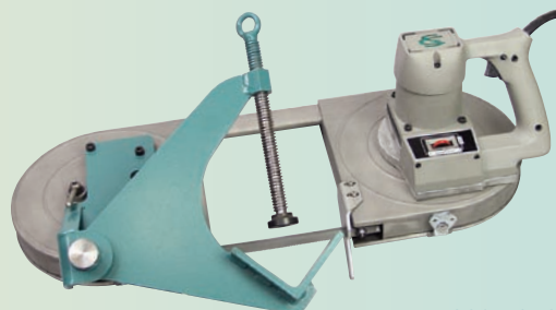
Model 5 6031 9400 with Band Saw
